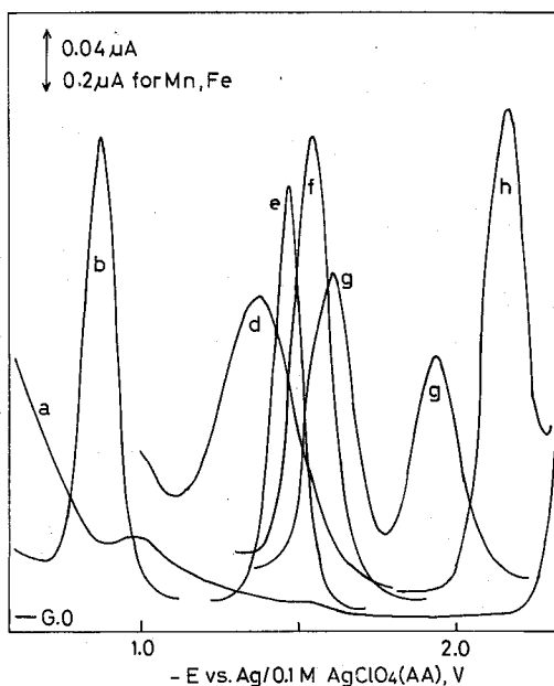
Fig. 5. Phase sensitive AC polarograms of metal acetylacetonates in non-aqueous AA. scan rate; 2 mV/sec, \Delta E ; 10 mV, t; 2.0 sec, 0.4 mM M-AA (0.2 mM for CuAA 2 ) in 0.1 M TBAP-AA solution, (a) residual current, (b) MnAA 3 , (d) CoAA 3 , (e) FeAA 3 , (f) CuAA 2 , (g) UO 2 AA 2 , (h) NiAA 2 .
