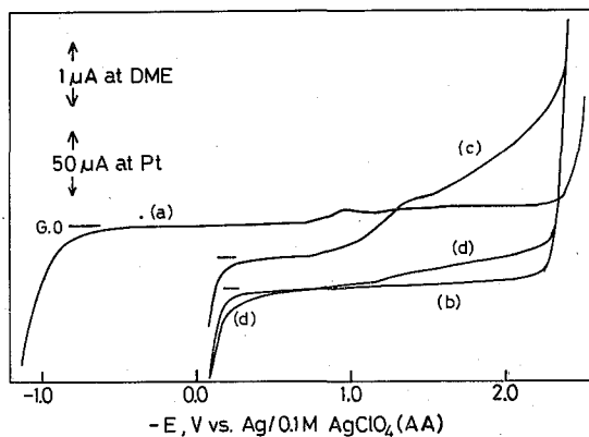
Fig. 1. Background DC polarograms in 0.1 M TBAP-acetylacetonone solution. (a) at stationary Pt wire electrode, (b) at DME in distilled AA, (c) at DME in commercial AA, (d) at DME in AA distilled by Freiser method.
