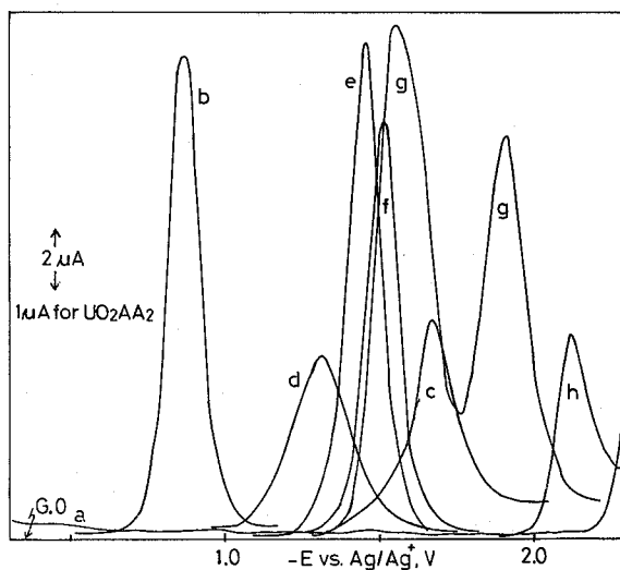
Fig. 4. Differential pulse polarograms of metal acetylacetonates in non-aqueous AA. scan rate; 2 mV/sec, modulation amplitude; 50 mV, t; 2.0 sec, 0.4 mM M-AA (0.2 mM for CuAA 2 ) in 0.1 M TBAP-AA solution, (a) residual current, (b) MnAA 3 , (c) PbAA 2 , (d) CoAA 3 , (e) FeAA 3 , (f) CuAA 2 , (g) UO 2 AA 2 , (h) NiAA 2 .
