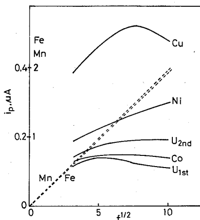
Fig. 6. Variations of PSAC peak currents with frequency. scan rate; 5 mV/sec, ΔE; 10 mV, 0.4 mM M-AA in 0.1 M TBAP-AA solution.
