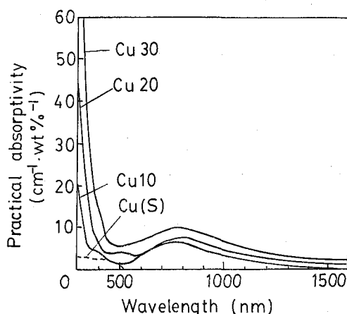
Fig. 18. Optical absorption spectra of CuO - SiO_2 films. Cu10: CuO 10 mol%, Cu20: CuO 20 mol%, Cu30: CuO 30 mol%, Cu(S): Schultz' data 37) .
