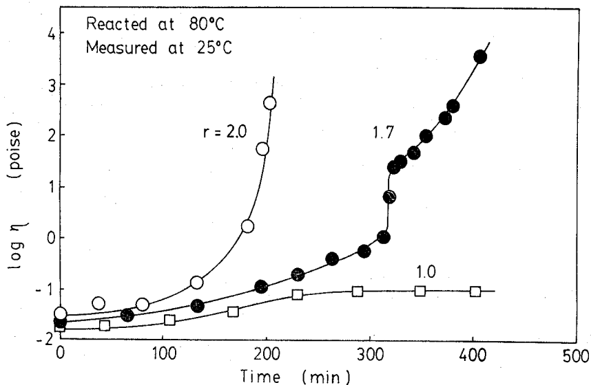
Fig. 8. Change of viscosity of \text{Si}(\text{OC}_2\text{H}_5)_4\text{-H}_2\text{O-C}_2\text{H}_5\text{OH} solution at 80°C. r = [\text{H}_2\text{O}]/[\text{Si}(\text{OC}_2\text{H}_5)_4] .
