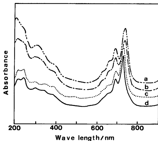
Fig. 1. UV/VIS spectra (in concd sulfuric acid) of films produced on copper film at 300°C (a), 350°C (b), 400°C (c) and 450°C (d).
