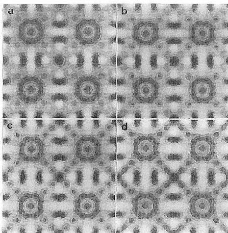
Fig. 9. Simulated images in the projection along the c -axis at various rotation angles: (a) 26°, (b) 27°, (c) 28°, (d) 29°.
