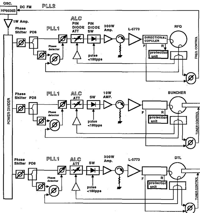
Fig. 4. RF control system
