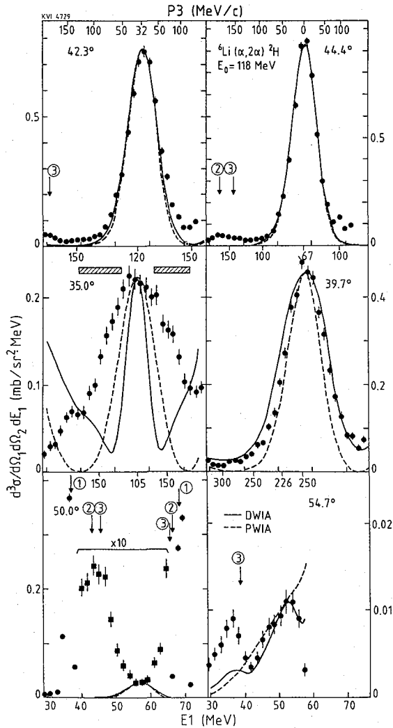
Fig. 1. Projected three body breakup cross sections for the {}^6\text{Li}(\alpha, 2\alpha){}^2\text{H} reaction at E = 118 MeV. Solid curves show the DWIA calculations and dashed curves the PWIA ones. Some arrows and hatched rectangles in the figure show the {}^6\text{Li} excitation energies. For details, see the text.
