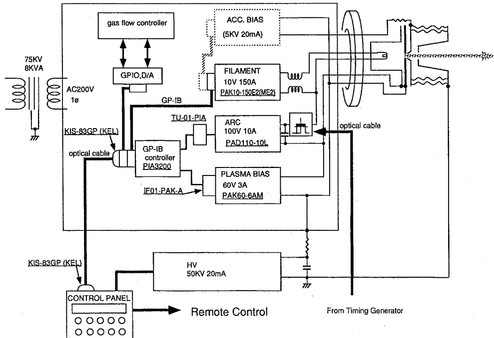
Fig. 1. Block diagram of the newly fabricated power supply capable of pulse-mode operation for the ion source.
