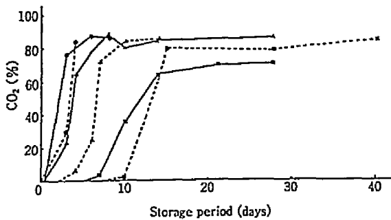
Fig. IV-12 Changes in concentration of carbon dioxide in the pouches containing Saccharomyces cerevisiae inoculated media. — : control, ---- : with oxygen-absorber. ● : Aw 0.95, ▲ : Aw 0.93, ■ : Aw 0.91.
