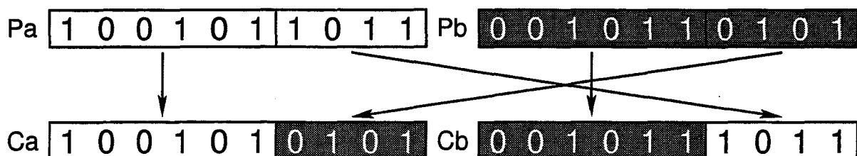
図 1.2: 一点交叉 Figure 1.2: One-point crossover
