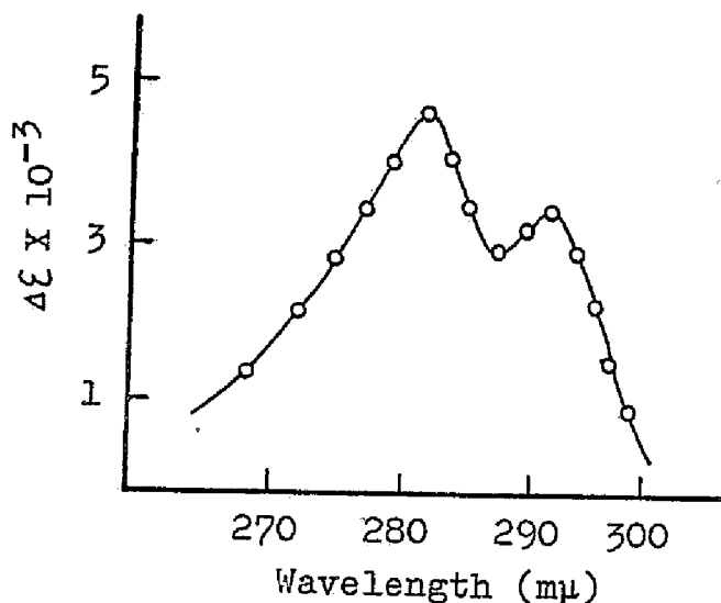
Fig. 14. Solvent Perturbation Difference Spectrum of PGA Mutase due to 20 % Polyethylene Glycol.
