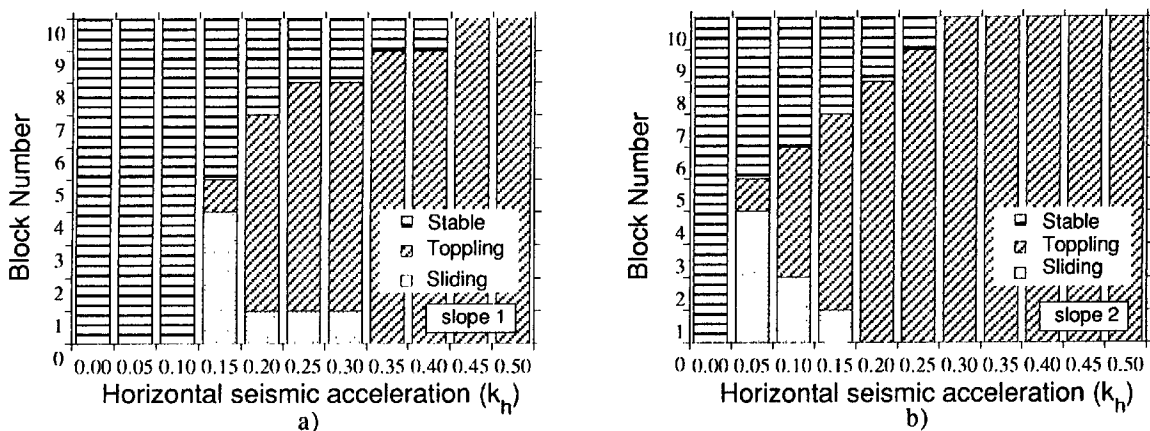
Fig. 12 Behavior type of each block at limiting equilibrium condition ( a ) ~ b ) )
