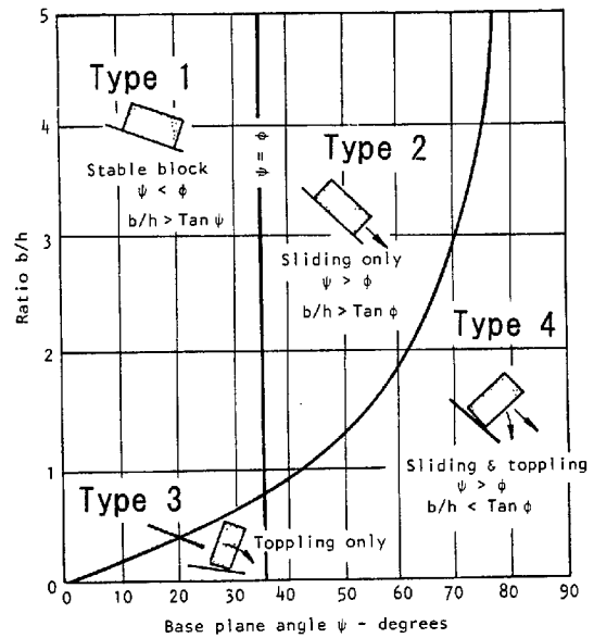
Fig. 5 Conditions for sliding and toppling of a block on an inclined plane (Hoek and Bray, 1981)
