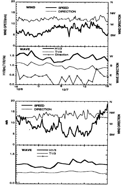
Fig.4 Wind and wave conditions at Case(1) & Case(2)
