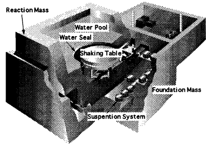
Fig.2 Schematic of Under Water Seismic Table
