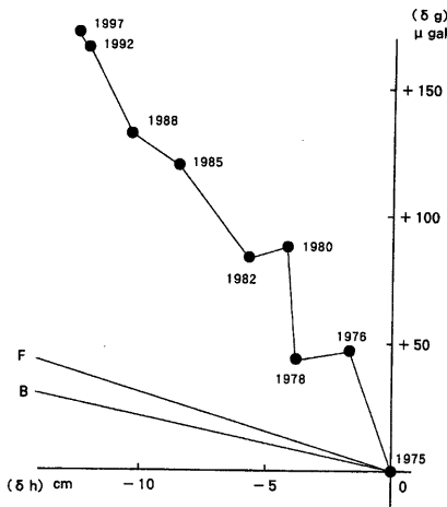
Fig. 5 Relation between relative gravity change and relative vertical displacement at BMSVO, taking the reference point of S16 located in western coast of Sakurajima.
