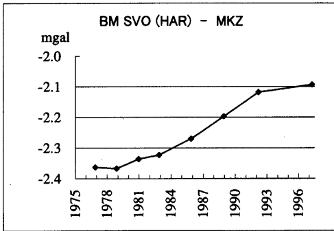
Fig. 4 Relative gravity change at BMSVO located on western flank of Sakurajima volcano, to the reference point of MKZ.
