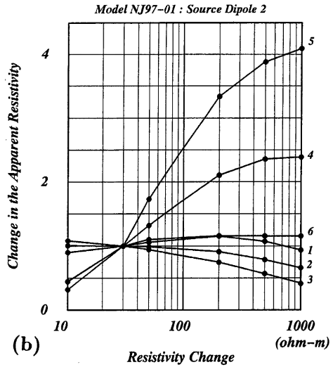
Fig. 5 : (a) Source Dipole 2 and 6 receiver dipoles, (b) resistivity changes observed with the receiver dipoles of Nos.1 to 6.
