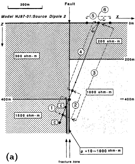
Fig. 5 : (a) Source Dipole 2 and 6 receiver dipoles, (b) resistivity changes observed with the receiver dipoles of Nos.1 to 6.
