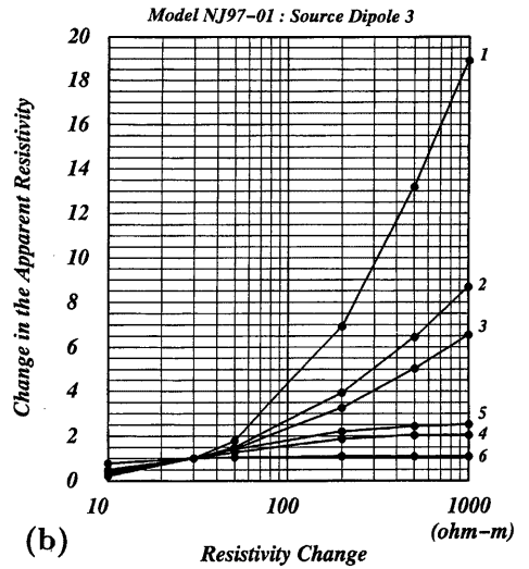
Fig. 6 : (a) Source Dipole 3 and 6 receiver dipoles, (b) resistivity changes observed with the receiver dipoles of Nos.1 to 6.
