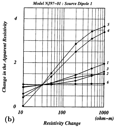
Fig. 4 : (a) Source Dipole 1 and 6 receiver dipoles, C: current electrodes, (b) resistivity changes observed with the receiver dipoles of Nos.1 to 6. Changes plotted in the figure are normalized with the apparent resistivity values when the resistivity of the fracture zone is 30\Omega m .
