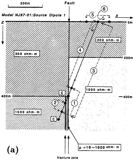
Fig. 4 : (a) Source Dipole 1 and 6 receiver dipoles, C: current electrodes, (b) resistivity changes observed with the receiver dipoles of Nos.1 to 6. Changes plotted in the figure are normalized with the apparent resistivity values when the resistivity of the fracture zone is 30\Omega m .
