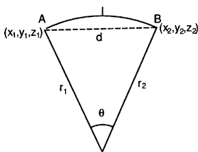
Fig. 12 Relation between chord ( d ) and arc ( l )
