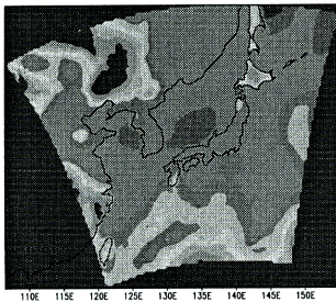
Fig. 32 Distribution of latent heat flux
