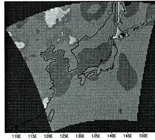
Fig. 33 Distribution of sensible heat flux
