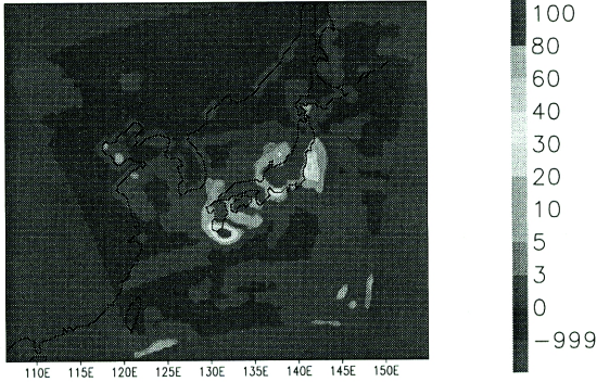
Fig. 28 Distribution of daily total rainfall and runoff
