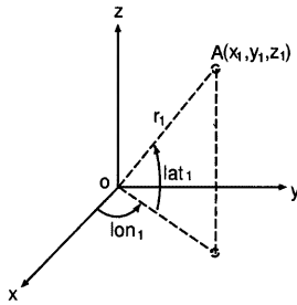
Fig. 11 Coordinate system on the earth's surface
