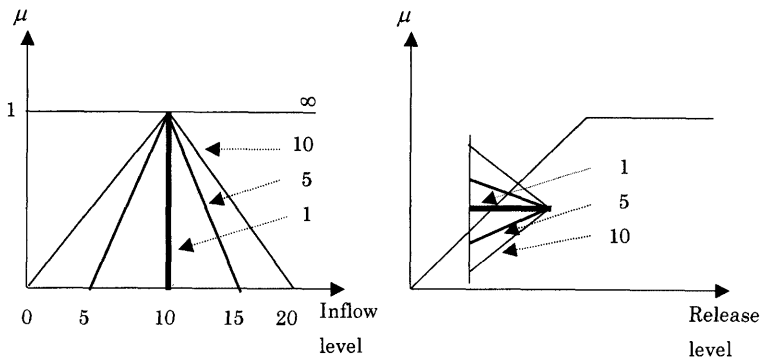
(a) fuzziness of inflow prediction (b) fuzziness of decision criteria Fig. 3 Selected types of fuzziness of inflow prediction and decision criteria for application
