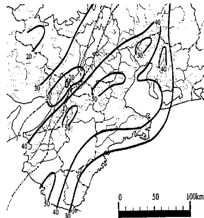
Fig. 8 Distribution of maximum instantaneous wind speed
