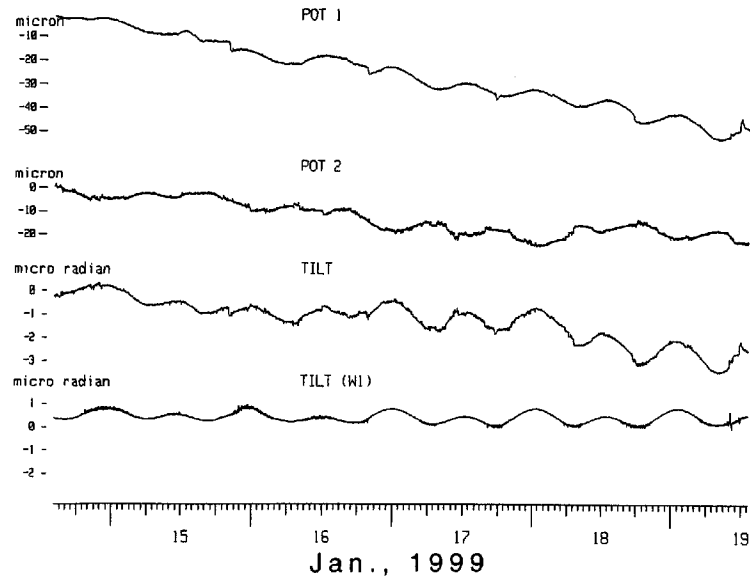
Fig.5 Record of test observation at entrance tunnel in Miyazaki observatory vault by type III instrument. (from top to bottom: POT1 level, POT2 level, tilt and record of routine tilt observation in the same direction in the observatory by type I instrument.)
