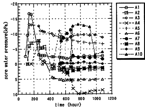
Fig. 3 In situ behavior of pore water pressure
