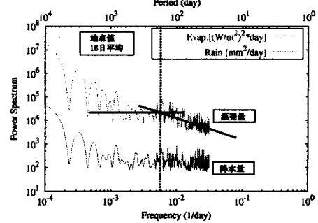
Fig. 23 Power spectra of time series of time-averaged point rainfall and evaporation
