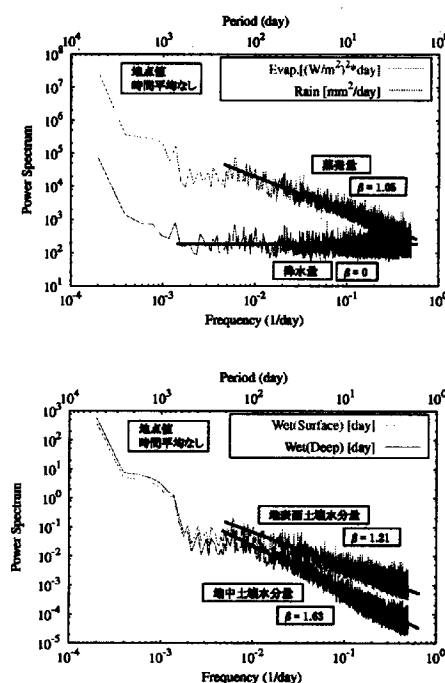
Fig. 25 Power spectra of daily rainfall and daily evaporation without areal averaging
