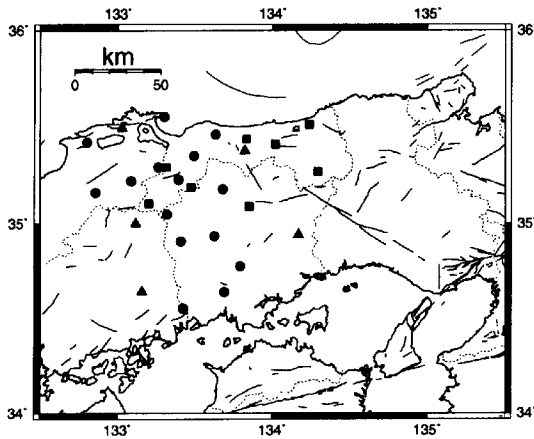
Fig. 6 Seismic stations used for locating hypocenters. There are 28 stations plotted. They consists of 8 DPRI stations, 5 JMA stations and 15 Hi-net stations.
