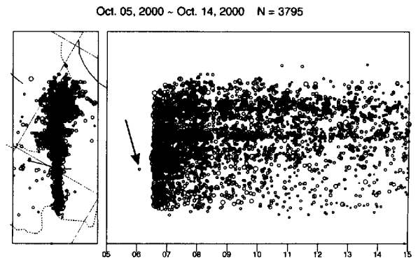
Fig. 14 (b) Foreshock that occurred 12 hours prior to the mainshock on the time-space plot. The foreshock is pointed by an arrow.
