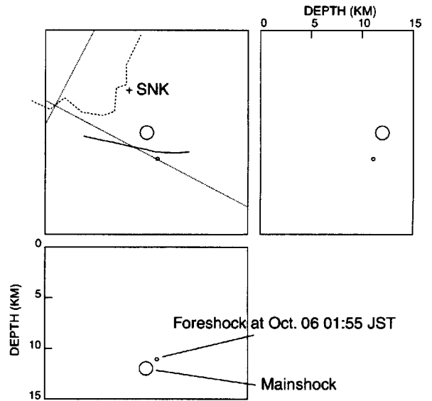
Fig. 14 (a) Location of the foreshock that occurred 12 hours prior to the mainshock. It is located using master event method with the mainshock.
