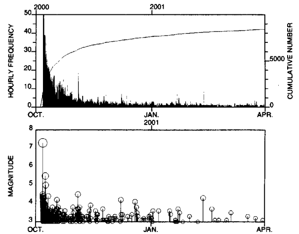
Fig. 11 Change of aftershock activity with time. Hourly frequency (upper, histogram), cumulative number (upper, line), and M-T diagram (lower) of the aftershocks shown in Fig.9. Preliminarily determined hypocenter catalogue by JMA is used to make the M-T diagram.
