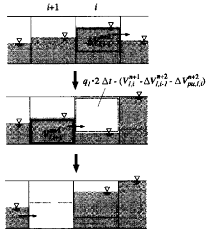
Fig.4 Computational process in a main sewer
