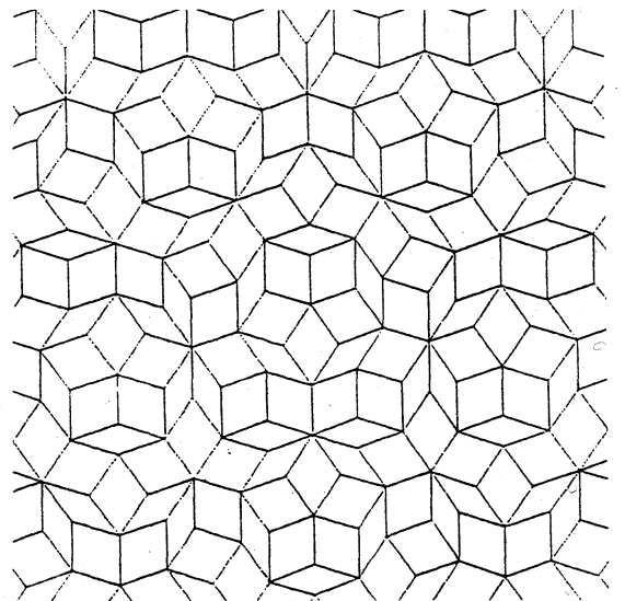
図2 Penrose Tiling
