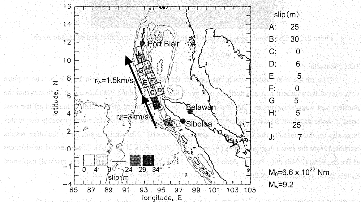
Fig. 2. 5 The slip distribution of the 2004 Sumatra-Andaman earthquake
