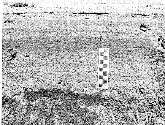
Photo 9 Tsunami deposits, sands, in the trenches along the survey line at Lhok Nga.
