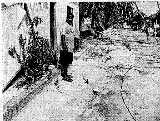
Photo 5.25 Sand erosion by tsunamis. Spacing red arrow indicates thickness of sands eroded by tsunamis.
