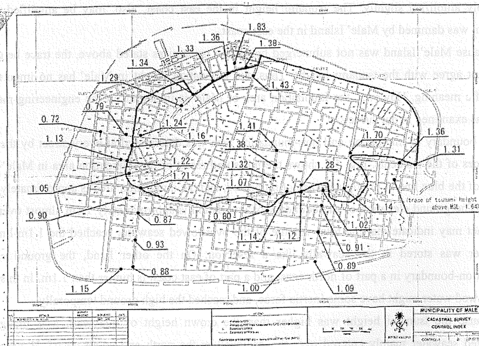
Fig. 5.2 Inundation area in Male' and the ground elevation near the boundary of inundation
