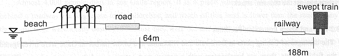
Fig. 3 Cross section of the damaged area, Kahawa, where the train was washed away
