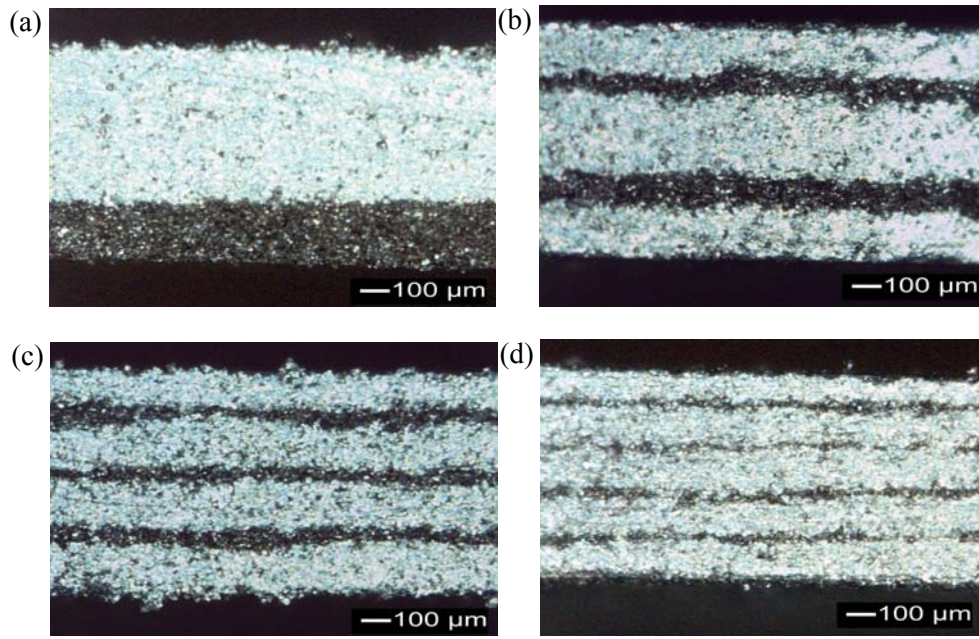
Fig. 6. Cross section images of multilayer samples C/G=10/90 using particle sized 25–32 \mu\text{m} with the number of layer of a 2; b 5; c 7; and d 9. The meaning of sample name of C/G=10/90 is given in Fig. 1 caption
