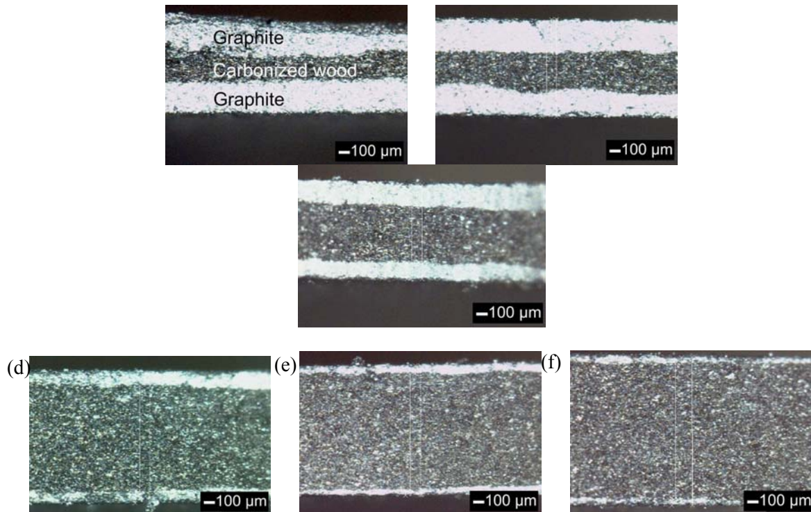
Fig. 1. Cross-section images of three-layer C/G composites using particle with the size of 25–32 \mu\text{m} in relation to weight fraction of carbonized wood: C/G = 10/90 ( a ); C/G=20/80 ( b ); C/G=33/67 ( c ); C/G=40/60 ( d ); C/G=70/30 ( e ); and C/G=80/20 ( f ). Sample name shows weight fractions of carbonized wood and graphite used. For example, C/G=10/90 means the sample contains 10 wt% of carbonized wood and 90 wt% of graphite
