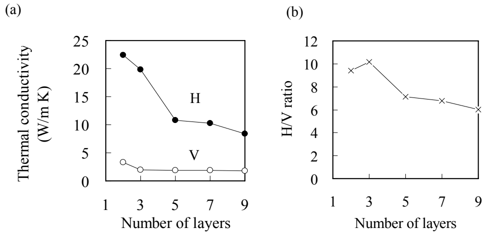
Fig. 5. Relation between number of layers with (a) thermal conductivity and (b) H/V ratio of samples C/G=10/90 using particle size of 25–32 \mu\text{m} . Filled circles , thermal conductivity in the horizontal direction (H); open circles , that of in the vertical direction (V); diagonal crosses , H/V ratio. The meaning of sample name of C/G=10/90 is given in Fig. 1 caption
