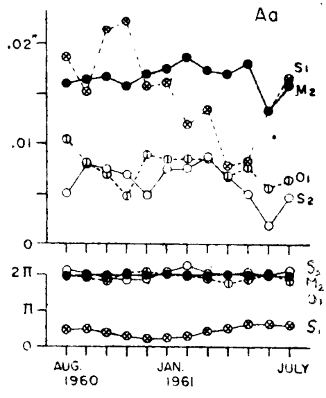
Fig. 9d. Amplitudes and phases of the E-W component tilt at Akibasan.
