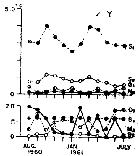
Fig. 9b. Amplitudes and phases of the air temperature observed at the Wakayama Meteorological Observatory.
