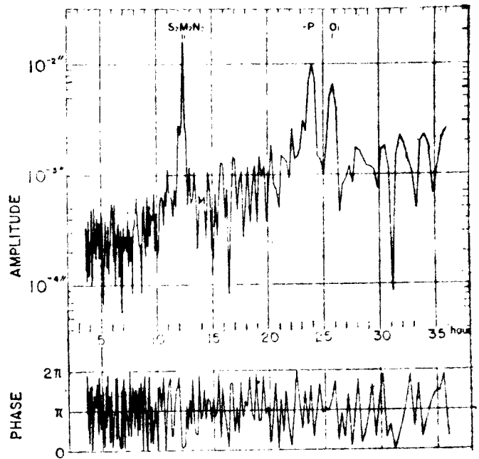
Fig. 11. Amplitude and phase spectra of the E-W component tilt ( Aa ) at Akibasan.
