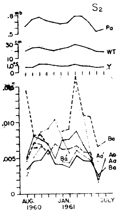
Fig. 10b. Comparison of the amplitudes in respect of S_2 .
