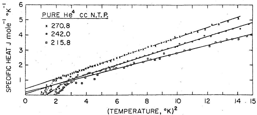
第2図 The specific heat of 0.90, 1.00, and 1.13 fractional monolayers of \text{He}^4 . Specific heat in J per mole per ^\circ\text{K} is plotted vs. the temperature squared in (^\circ\text{K})^2 . (Brewer 2 )による)
