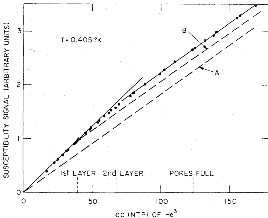
第6図 He 3 nuclear resonance signal plotted against quantity of sample. (Brewer 1) による)
