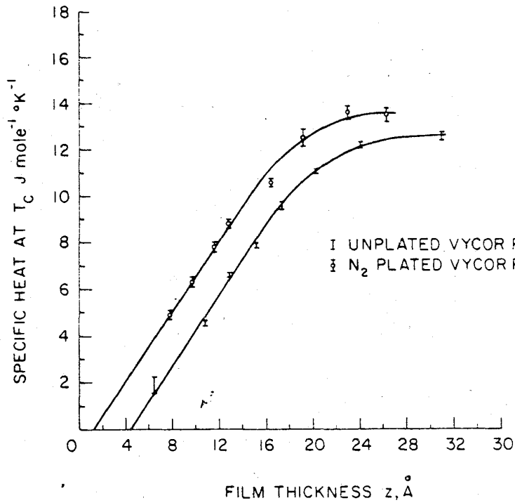
第5図 Variation of the specific heat of the He 4 film at the maximum in the anomaly as a function of film thickness. (Brewer 1) による)
