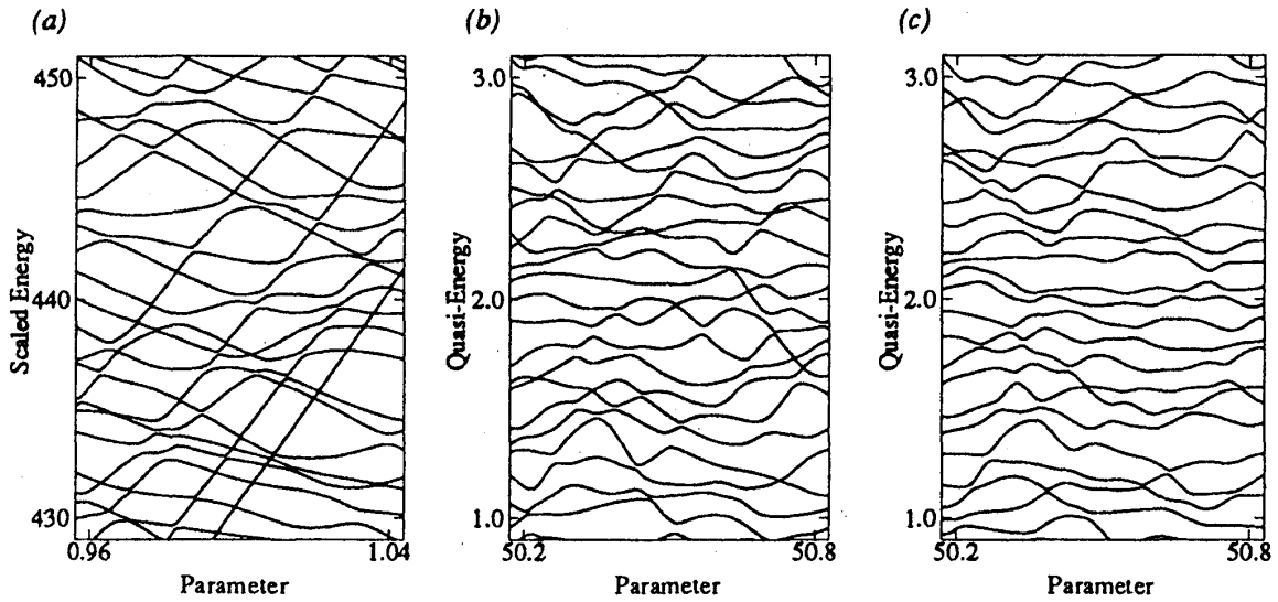
Fig.1 The parametric motion of eigenvalues or quasi-eigenvalues: (a) stadium billiard; (b) kicked rotator with time-reversal symmetry ( N = 64, M = 1, a = 1/\sqrt{2}, b = 0 ); (c) kicked rotator without time-reversal symmetry ( N = 64, M = 1, a = 1/\sqrt{2}, b = \sqrt{3} ).
