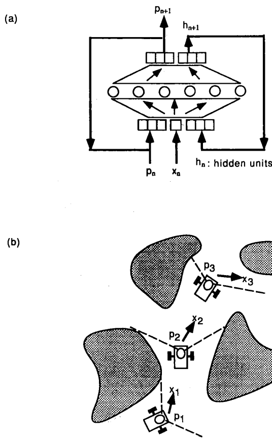
Figure 3: (a) is an RNN architecture for forward modeling, (b) is schematics of how a robot obtains sensori-motor sequences.
