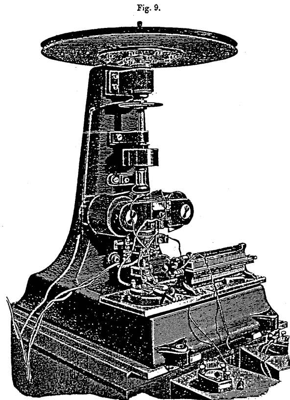
Whirling machine for ether experiment, with pair of steel disks, 1 yard in diameter. From a photograph taken during preliminary tests, before it was bolted down to stone pier. Full voltage is always supplied to the field magnets, variable resistance is in armature circuit only. The brass tube conducts away surplus oil. Drawings of the machine are given in Plate 32.
