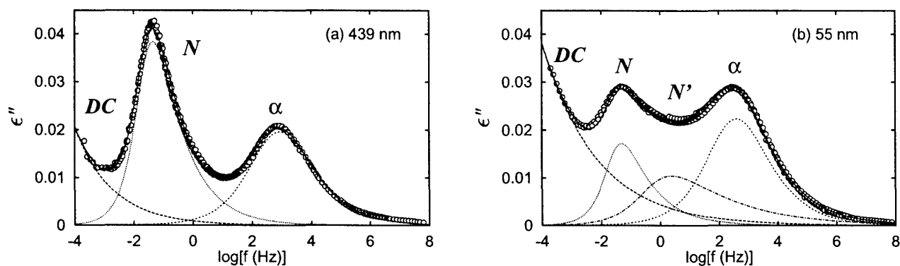
Fig.2: Master curves for dielectric loss as a function of frequency for thin films of PI with M_n=1.0\times 10^4 for various film thickness: (a) d=439 nm, (b) d=55 nm. The reference temperature T_r is 229K. The original data are measured over the temperature range from 205 K to 308 K.
