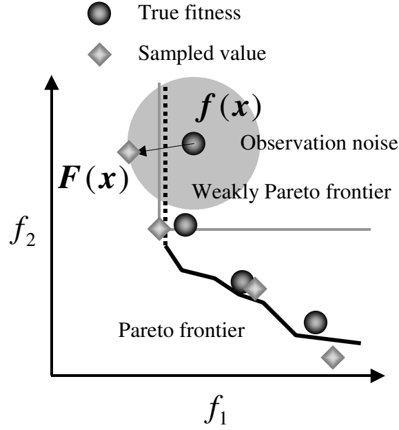
Figure 4.1: A weakly Pareto individual treated as a non-dominated individual.
