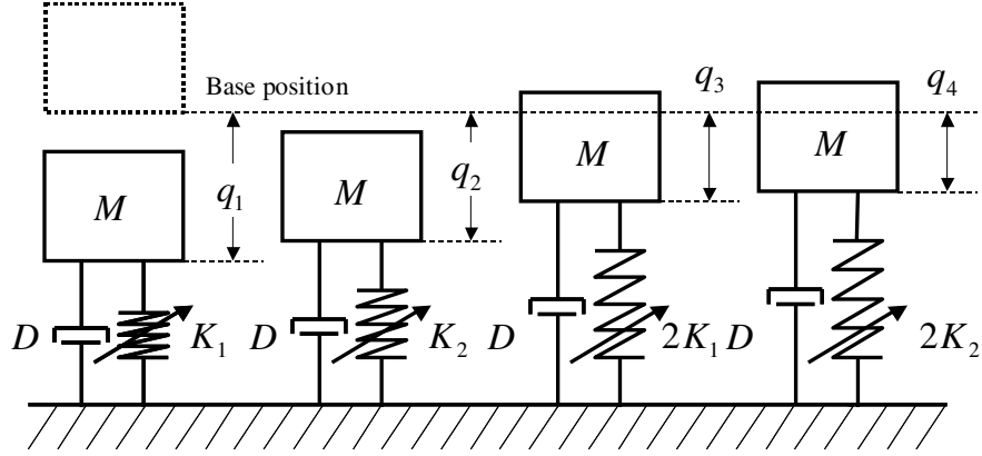
Figure 6.8: Mass-damper-spring system.
