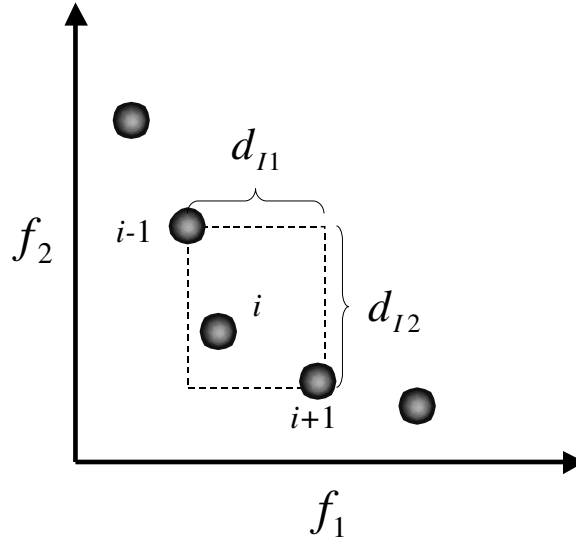
Figure B.2: Calculation of crowding distance.
