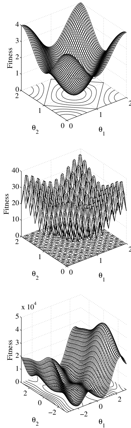
Figure 5.6: Shape of the periodic test functions (upper: Periodic Unimodal, middle: Periodic Multimodal, lower: Fletcher and Powell (2-dimension)).
