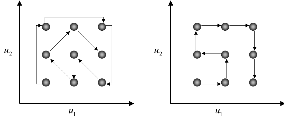
Figure 8.9: Scheduling of condition variable vectors (left: Type A, right: Type B).
