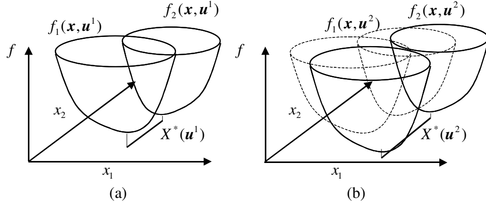
Figure 8.2: Schematic diagram of MOPs with condition variables.
