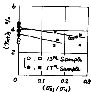
Fig. 8 \gamma_{oet} at Failure plotted to Principal Stress Ratio
