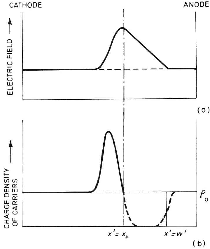
Fig. 6.3 Distribution of electric field (a) and charge density of carriers (b) in transferred-electron diode with complete depletion of carriers in leading edge.
