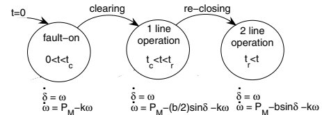
Figure 1: Switching sequence governing the SMIB system with clearing and re-closing operations.
