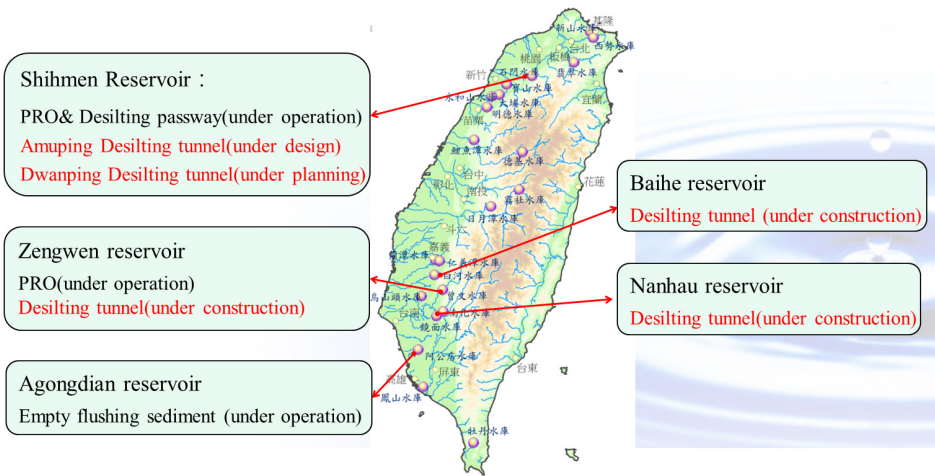
Figure 3: Hydraulic desilting projects in major reservoirs
