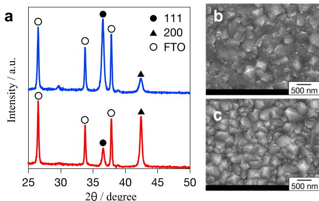
Figure 4. (a) XRD patterns and (b), (c) SEM images of \text{Cu}_2\text{O} obtained from the electrodeposition bath with c_{\text{NaOH}} = 3.8 M. These data confirm that \text{Cu}_2\text{O} was obtained immediately after preparation of the bath (blue, b) and after thermodynamic equilibration following aging for one day (red, c). Each scale bar indicates 500 nm.
