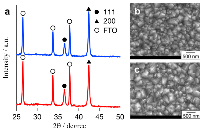
Figure 5. (a) XRD patterns and (b), (c) SEM images of \text{Cu}_2\text{O} obtained from the electrodeposition bath prepared by adding an excess of sodium hydroxide ( c_{\text{NaOH}} = 4.0 M) followed by partial neutralization using 0.3 M acetic acid. These data confirm that \text{Cu}_2\text{O} was obtained immediately after preparation of the bath (blue, b) and after reaching the thermodynamic equilibrium through 24 h aging of the bath (red, c). Each scale bar indicates 500 nm.
