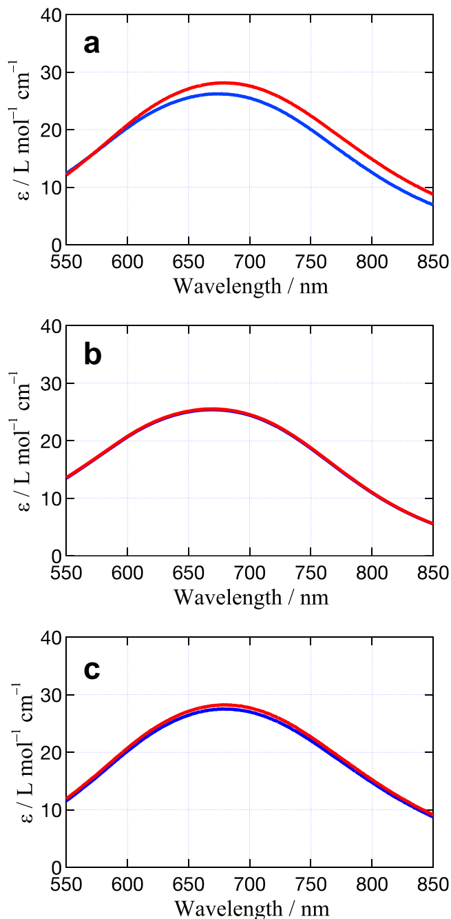
Figure 3. Visible absorption spectra of \text{Cu}_2\text{O} electrodeposition baths having (a) c_{\text{NaOH}} = 3.8 \text{ M} and (b) c_{\text{NaOH}} = 4.0 \text{ M} and (c) prepared by adding an excess of sodium hydroxide ( c_{\text{NaOH}} = 4.0 \text{ M} ) followed by 0.3 \text{ M} acetic acid to partially neutralize the sodium hydroxide. The blue and red lines indicate values immediately after preparation of the bath and after reaching thermodynamic equilibrium following aging of the bath for one day, respectively.
