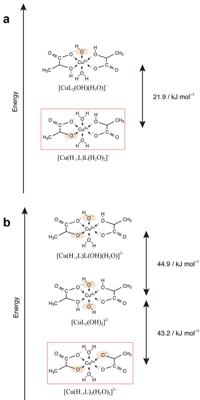
Figure 2. Structures and energy differences of (a) a complex with one proton dissociated and (b) complexes with two protons dissociated from [CuL 2 (H 2 O) 2 ] 0 .
