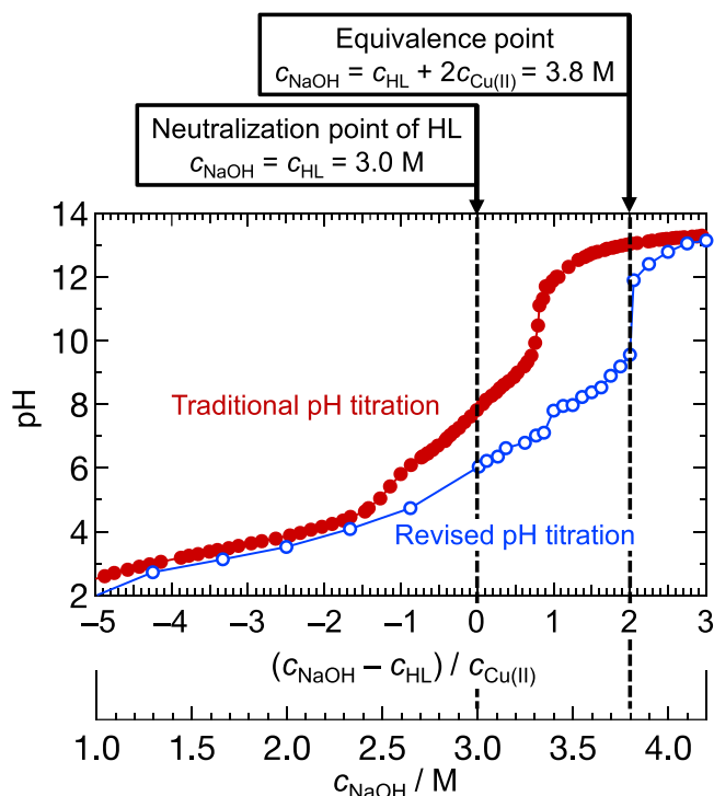
Figure 1. Titration curves for an aqueous 0.4 M copper(II)/3.0 M lactate solution with added NaOH. The dashed lines indicate neutralization and equivalence points. The plots corresponding to traditional and revised pH titrations are depicted in red and blue, respectively. (The titration data was reproduced from Ref. 11).
