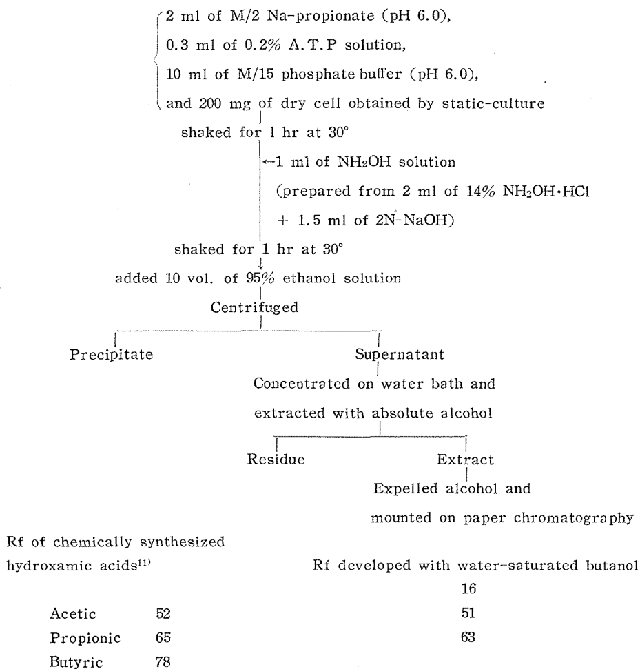
Fig. 4. The formation of hydroxamates in the propionate oxidation.
