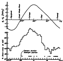
Figure 6.11: The upper plot gives difference in magnetic field strength at 300 km at conjugate points along 65^\circ invariant latitude. The lower plot gives occurrence of aurora observed on all-sky camera from auroral stations located between 64^\circ and 70^\circ N geomagnetic latitude [Stenbaek-Nielsen et al., 1971].
