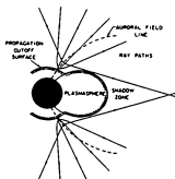
Figure 6.2: Qualitative sketch of the ray paths of AKR at low altitudes and fixed frequency along an auroral field line. Because the refractive index goes to zero at the propagation cutoff, there is a strong tendency for the ray paths to be refracted upward, away from the propagation cutoff surface [Gurnett, 1974].
