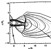
Figure 7.6: The trajectory of SL-9 (thick and dashed line) in the meridian plane projection [Hordnyi, 1994]. Plasma density contours (thin lines) mark the values of n_p = 10^{-2}, 10^{-1}, 10^0, 10^1, 10^2, 10^3 \text{ cm}^{-3} and the magnetic field lines shown (dotted lines) pierce the magnetic equator at L = 2, 4, 6, \dots R_J .
