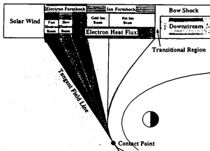
Figure 1.4: Structure of the terrestrial foreshock region [Matsumoto et al. , 1997].
