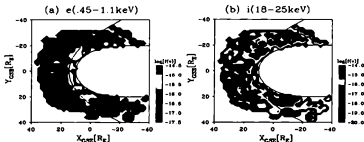
Figure 3.13: Global distributions of energetic particles with velocities parallel to the local IMF orientation. (a) electrons in 0.45–1.1 keV ( \text{s}^2/\text{m}^6 ); (b) ions in 18–25 keV ( \text{s}^2/\text{m}^6 ).
