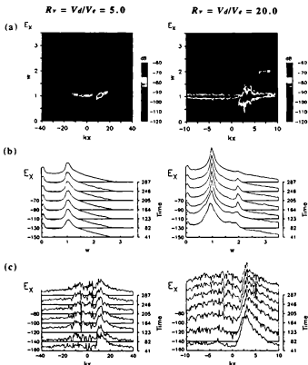
Figure 4.7: Plasma waves in E_x (dB) in the simulation runs with R_v = V_d/V_e = 5.0 (left) and 20.0 (right), keeping R_m = 1/1600 and R_n = 0.02 . (a) the \omega - k_x diagram in t = 82 –246; (b) evolution of plasma waves in \omega space; (c) that in k_x space with \omega = 0.5 –2.5 in E_x and \omega = 1.75 –2.25 in B_z .
