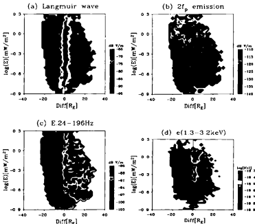
Figure 3.16: Activities of plasma waves and energetic particles correlated with kinetic energy flow in the solar wind, n_{sw} m_e v_{sw}^3 ( \text{mW}/\text{m}^2 ), observed from November 1994 to April 1996. X-axis is \text{Diff} , and Y-axis is \log(n_{sw} m_e v_{sw}^3) , respectively. (a) Langmuir wave; (b) 2f_p radiation; (c) electric field in 24-196 Hz; (d) electrons in 1.3-3.2 keV.
