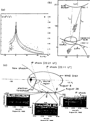
Figure 2.1: Previous results to determine the 2f_p radio source. (a) Flux of the 2f_p radiation associated with passage of ISEE-1 through the electron foreshock region. X-axis is distance from the tangential IMF line projected to the Sun-Earth line. Y-axis is flux of 2f_p radiation [Lacombe et al. , 1988]. (b) The direction finding result by ISEE 3 associated with density jump in the solar wind [Hoang et al. , 1981]. (c) The direction finding result by WIND associated with density jump in the solar wind [Reimer et al. , 1996].
