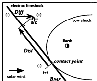
Figure 3.1: Geometry of the terrestrial foreshock [cf. Filbert and Kellogg, 1979; Etcheto and Faucheux, 1984 ].
