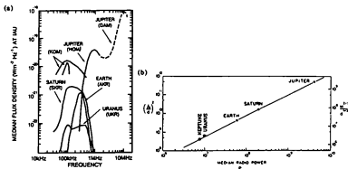
Figure 7.2: Planetary AKR-like radio emissions. (a) The median flux density observed by Voyager PRA instrument from a distance of 1 A.U. from each planet [Kaiser, 1989]; (b) The “radiometric Bode’s law”, the relation between the total solar wind input power into the magnetospheres and the total radio power of planetary AKR-like radio emissions. Efficiency of energy conversion is about 5 \times 10^{-6} [Desch and Kaiser, 1984].
