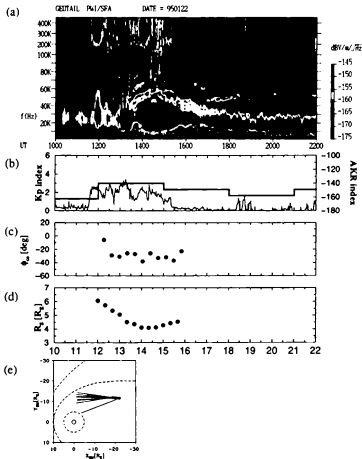
Figure 5.13: Continuum enhancement observed on 22 January 1995. (a) Frequency-time diagram of the PWI/SFA; (b) Kp index (thick line) and AKR index (thin line); (c) Azimuth angle ( \phi_{cc} ) at 40 kHz; (d) Radial distance of the source ( R_s ); (e) Observed location and \phi_{cc} at 40 kHz from 12–16h UT on the SM coordinates.
