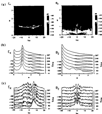
Figure 4.3: Plasma waves in E_x (left) and B_z (right) in the standard run with R_m = 1/1600 , R_v = 10.0 , R_n = 0.02 . (a) the \omega - k_x diagram in t = 82 -240; (b) evolution of plasma waves in \omega space; (c) that in k_x space with \omega = 0.5 -2.5 in E_x and \omega = 1.75 -2.25 in B_z . Electric and magnetic field is indicated in dB.
