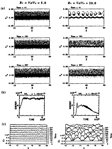
Figure 4.6: Evolution of particles and electric field in the simulation runs with R_r = V_d/V_e = 5.0 (left) and 20.0 (right), keeping R_m = 1/1600 and R_n = 0.02 . (a) Phase diagrams of particles in x - v_x ; (b) Total energy of electric field; (c) Spatial structure of electric field E_x along X -axis.
