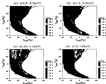
Figure 3.15: The mappings of the energetic particles with velocities parallel to the local IMF orientation in the terrestrial foreshock observed from November 1994 to April 1996. Plots are using normalized foreshock coordinates on a common diagram of the nominal IMF at 120^\circ stream angle and nominal shock. (a) electrons in 3.8-9.3 keV; (b) electrons in 1.3-3.2 keV; (c) electrons in 0.45-1.1 keV; (d) ions in 12-16 keV.
