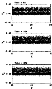
Figure 4.10: Evolution of particles and electric field in the 2D simulation run with R_m = 1/1600 , R_v = 10.0 , R_n = 0.02 . (a) Phase diagrams of particles in x-v_x ; (b) Total energy of electric field;
