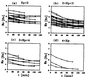
Figure 5.15: Variations of radial distance of the source from the Earth ( R_s ) classified by Kp index; (a) Kp < 2 , (b) 2 \leq Kp < 3 , (c) 3 \leq Kp < 4 , and (d) 4 \leq Kp . X-axis is time after the onset of each substorms, and Y-axis is distance of the source from the Earth ( R_s ).
