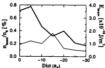
Figure 3.20: Densities (thick line) and kinetic energies (thin line) of quasi-beam components observed at leading edge of upstream wing of the electron foreshock. X-axis is Dist of observed locations. Left and right Y-axis indicates density ratio (%) and kinetic energy ( \text{J/m}^3 ) of the quasi-beam component.
