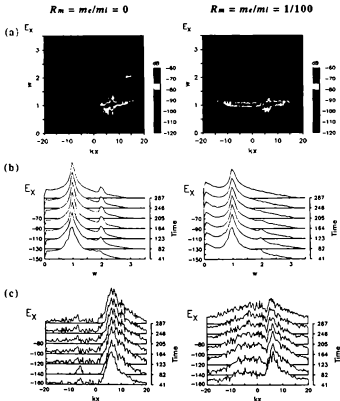
Figure 4.5: Plasma waves in E_x (dB) in the simulation runs with R_m = m_e/m_i , = 0 (left) and 1/100 (right), keeping R_v = 10.0 and R_n = 0.02 . (a) the \omega - k_x diagram in t = 82 -246; (b) evolution of plasma waves in \omega space; (c) that in k_x space with \omega = 0.5 -2.5 in E_x and \omega = 1.75 -2.25 in B_x .
