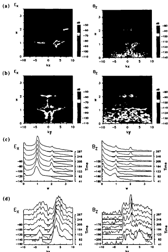
Figure 4.11: Plasma waves in E_x (left) and B_z (right) in the 2D simulation run with R_m = 1/1000 , R_v = 10.0 , R_n = 0.02 . (a) the \omega - k_x diagrams along X-axis in t = 82 -246; (b) the \omega - k_y diagram along Y-axis in t = 82 -246; (c) evolution of plasma waves in \omega space; (d) that in k_x space with \omega = 0.5 -2.5 in E_x and \omega = 1.75 -2.25 in B_z .
