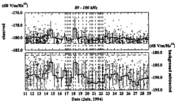
Figure 7.11: Background-noise subtracted fluxes from the Jovian direction in July 11-28, 1994. They are the 1-minute averaged values, Y-axis is radiation flux ( \text{dB V m}^{-1} \text{Hz}^{-1/2} ). Only the data in which the k vector direction is within \pm 15^\circ from the Jovian direction are indicated. Thick line shows the average over 12-hour intervals. 1\sigma value at every 12 hours is overlaid by thin vertical lines. Dashed vertical line shows the impacts time of all fragments. Long dashed horizontal line shows the background noise level. (a) Radiation flux at 712-800 kHz (HOM). Upper panel shows the observed data, and lower panel shows the background subtracted data. (b) Radiation flux at 89-100 kHz (KOM). Upper panel shows the observed data, and lower panel shows the background subtracted data.
