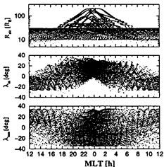
Figure 6.4: Trajectories of GEOTAIL from January 1993 to February 1996. (a) MLT and radial distance of GEOTAIL, R_{\infty} ; (b) MLT and magnetic latitude of GEOTAIL, \lambda_m ; (c) MLT of GEOTAIL and magnetic latitude of sub-solar point, \lambda_{sun} .
