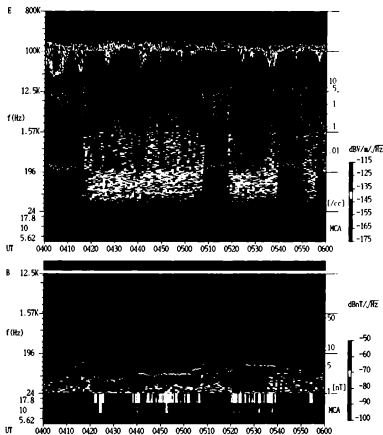
Figure 3.7: Plasma wave spectra around the bow shock observed by the SFA and MCA in 4–6h UT on 25 April 1995. White lines indicate electron gyrofrequency, f_g .
