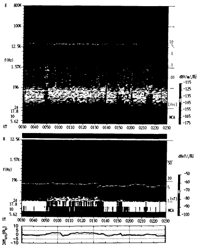
Figure 3.3: Plasma wave spectra around the electron foreshock observed by the SFA and MCA in 0:30-2:30 UT on 6 April 1995. White lines indicate electron gyrofrequency, f_g . Bottom column is Diff at GEOTAIL.
