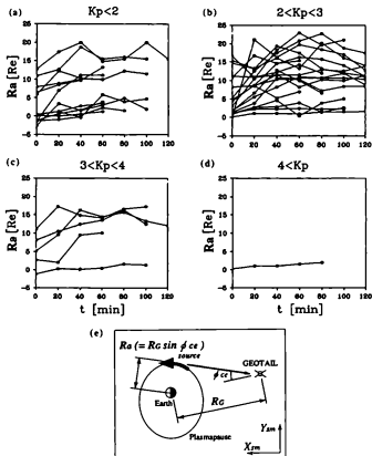
Figure 5.10: Variations of azimuth angle ( \phi_{cc} ) classified by Kp index; (a) K_p < 2 , (b) 2 \leq K_p < 3 , (c) 3 \leq K_p < 4 , and (d) 4 \leq K_p . X-axis is time after the onset of each substorms. Y-axis is the apparent distance of the source ( R_a ) defined from \phi_{cc} . Concept of relation between R_a and \phi_{cc} is indicated in (e).
