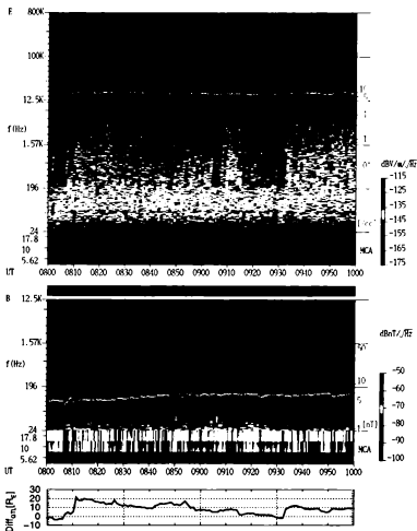
Figure 3.5: Plasma wave spectra around the ion foreshock observed by the SFA and MCA in 8–10h UT on 6 April 1995. White lines indicate electron gyrofrequency, f_g . Bottom column is \text{Diff}_B at GEOTAIL.
