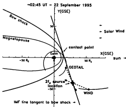
(a) 2f_p radio source located by WIND/GEOTAIL triangulation
