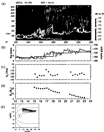
Figure 5.11: Continuum enhancement observed on 14 November 1994: (a) Frequency-time diagram of the PWI/SFA; (b) Kp index (thick line) and AKR index (thin line); (c) Azimuth angle ( \phi_{cr} ) at 40 kHz; (d) Radial distance of the source ( R_s ); (e) Observed location and \phi_{cr} at 40 kHz from 15-19h/21-23h UT on the SM coordinates.
