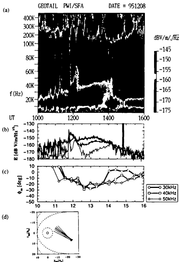
Figure 5.9: Continuum enhancement observed in 12–15 h UT on 8 December 1995. (a) Frequency–time diagram of the PWI/SFA; (b) Flux and (c) azimuth angle ( \phi_a ) at 30, 40, and 50 kHz in 20-minute interval. Origin of \phi_a is direction of the Earth; (d) Observed location and azimuth angle \phi_a at 40 kHz from 12–14 h UT on the SM coordinates.
