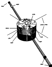
Figure 1.5: Configuration of the GEOTAIL spacecraft [Nishida, 1994].
