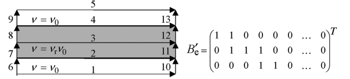
Fig. 3. Thin elements, in which material property changes discontinuously.
