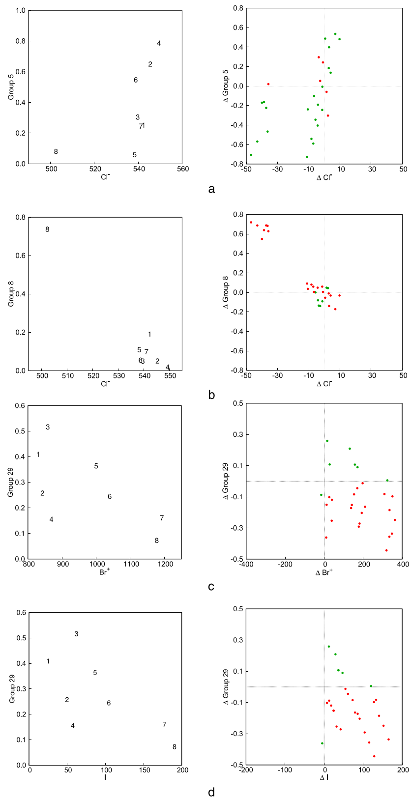
Figure 3. Scatterplots (a–d) of the pairs of the abundances of \text{Cl}^- , \text{Br}^+ , and \text{I} in the eight layers and the relative frequencies of the sequences in Groups 5, 8, and 29 in the eight layers (left) and of the pairs of the differences in the abundances of \text{Cl}^- , \text{Br}^+ , and \text{I} between the eight layers and the differences in the relative frequencies of the sequences in Groups 5, 8, and 29 between the eight layers (right).
