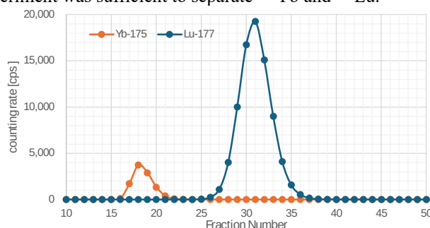
Fig. 2. Elution profile of extraction chromatography with an 11 mm \phi x 240 mmL column packed with LN2 resin measured with a Ge detector (Left) and a CZT detector (Right)
