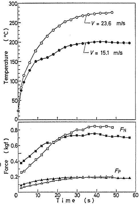
Fig. 6. Progress of cutting edge temperature, F_N and F_P with rubbing time at higher velocities, 15.1 and 23.6 m/s.
