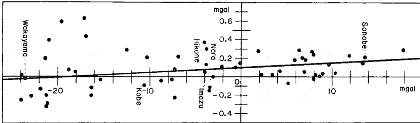
Fig. 2 The abscissa represents the gravity difference between each station and the base station, the ordinate the difference between the gravity value of the present survey and that of the former one at each station.
