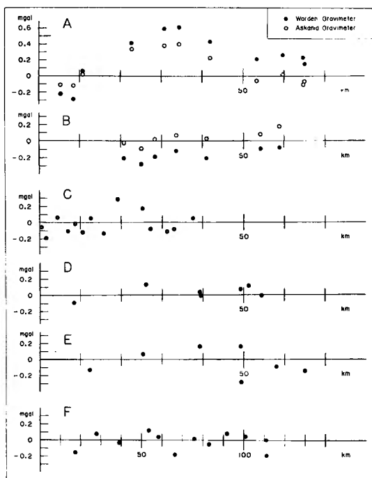
Fig. 3 Gravity change in each survey route. The abscissa represents the distance of each observation station from the base station.
