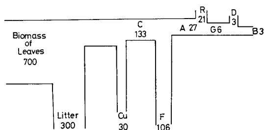
Fig. 9. Flow diagram of dry matter in the pine stand.
