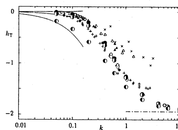
Fig. 15. Thermal force (2RT_0)^{-1/2} L^2 \lambda_g (\partial T / \partial X_i)_\infty h_T on a spherical particle with an arbitrary thermal conductivity: h_T vs k . Here, \bullet indicates the numerical result for \lambda_p/\lambda_g = \infty , \circ for 10, \circ for 1. The solid lines — indicate the asymptotic solutions for small k {from the top, \lambda_p/\lambda_g = \infty (correct up to O(k^2)^{10} ), 10 and 1 [Eq. (56)]}, and --- indicates the free molecular limit ( k \rightarrow \infty ) [Eq. (54)]. Experimental results by several authors are indicated by smaller markers: \times indicates the case \lambda_p/\lambda_g = 475 (Hg in Air), \Delta 263 (NaCl in Air), \blacktriangle 8.14 (tricresyl phosphate in Air) in Ref. 32; \nabla 366 (NaCl in Ar) in Ref. 34; \bullet 8.14 (tricresyl phosphate in Air) in Ref. 36; + 7.41 (Oil in Ar) in Ref. 30. Numerical results in Ref. 45 are also indicated by small markers: \diamond and \circ indicate \lambda_p/\lambda_g = 100 and 10 respectively.
