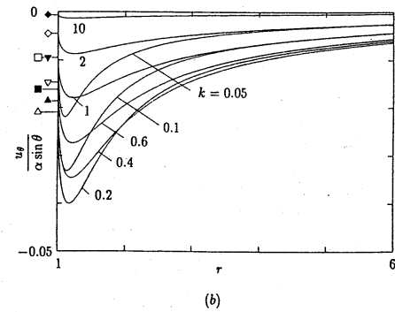
Fig. 4. Velocity field: (a) u_r/\alpha \cos \theta , (b) u_\theta/\alpha \sin \theta . Here, — indicates the present numerical result. The flow vanishes for the Stokes solution without slip ( k=0 ) and the free molecular solution ( k=\infty ). The values on the sphere are marked by \square for k=0.05 , \blacksquare for k=0.1 , \triangle for k=0.2 , \blacktriangle for k=0.4 , for \nabla k=0.6 , \blacktriangledown for k=1 , \diamond for k=2 , and \blacklozenge for k=10 in (b).
