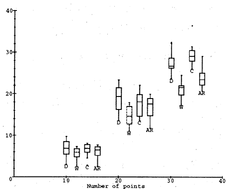
Figure 6: Weight of triangulations
