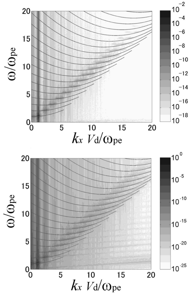
FIG. 1. Numerically simulated \omega – k_x diagram, which is generated by plotting the wave intensity, |E_x(\omega, k_x)|^2 , in grayscale versus \omega and k_x . In the first case, the data were collected over a time period ranging from \omega_{pe}t = 409.6 to \omega_{pe}t = 512.0 . The second case corresponds to 819.2 < \omega_{pe}t < 921.6 . The intensity is normalized by the thermal energy of the background electrons n_e m_e V_{te}^2/2 . The solid lines show the linear and nonlinear dispersion curves obtained from Eq. (8).
