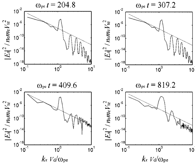
FIG. 7. Spectra of the normalized wave electric field energy, 2|E_x(k_x)|^2/n_e m_e V_{te}^2 , versus k_x V_d/\omega_{pe} , at \omega_{pe}t = 204.8, 307.2, 409.6 , and 819.2 . The dashed line represents the initial profile of the wave intensity. Note that the final spectrum is roughly characterized by the initial power-law index of \sim -5 .
