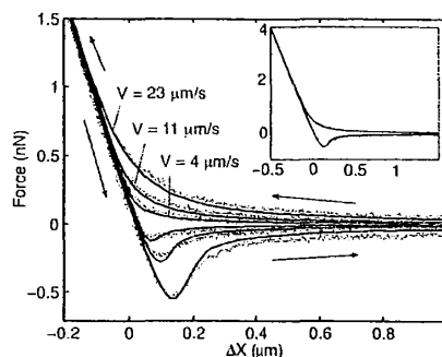
Fig 1b: AFM: Particle-Drop interaction [12]
