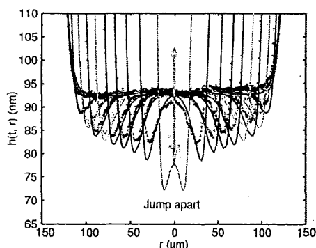
Fig 2b: SFA: Pull-off of a stable film [10]
