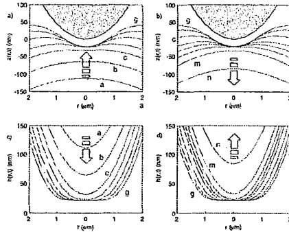
Fig 3b: AFM: Particle-Drop profile [12]
