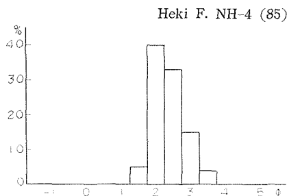
Fig. 3. Mechanical composition of a sandstone of the Heki Formation.
