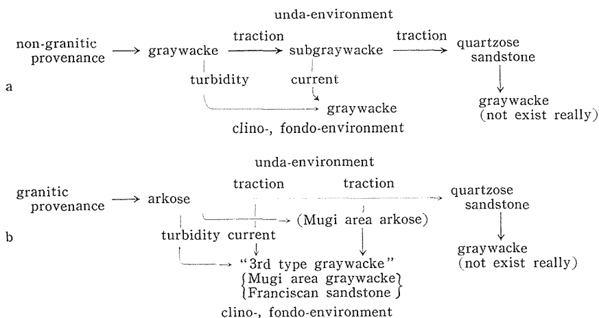
Figure 13 a &amp; b. Development of some sandy deposits when the basin is large.
