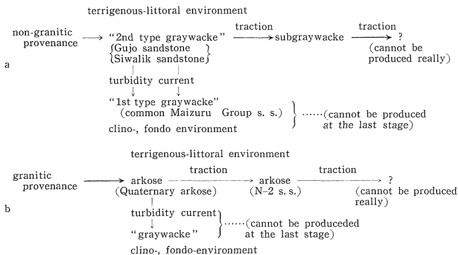
Figure 14 a &amp; b. Development of some sandy deposits when the basin is small.
