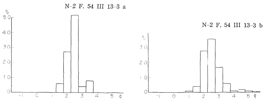
Figs. 2 a & b. Mechanical composition of sandstones of the N-2 Formation.
